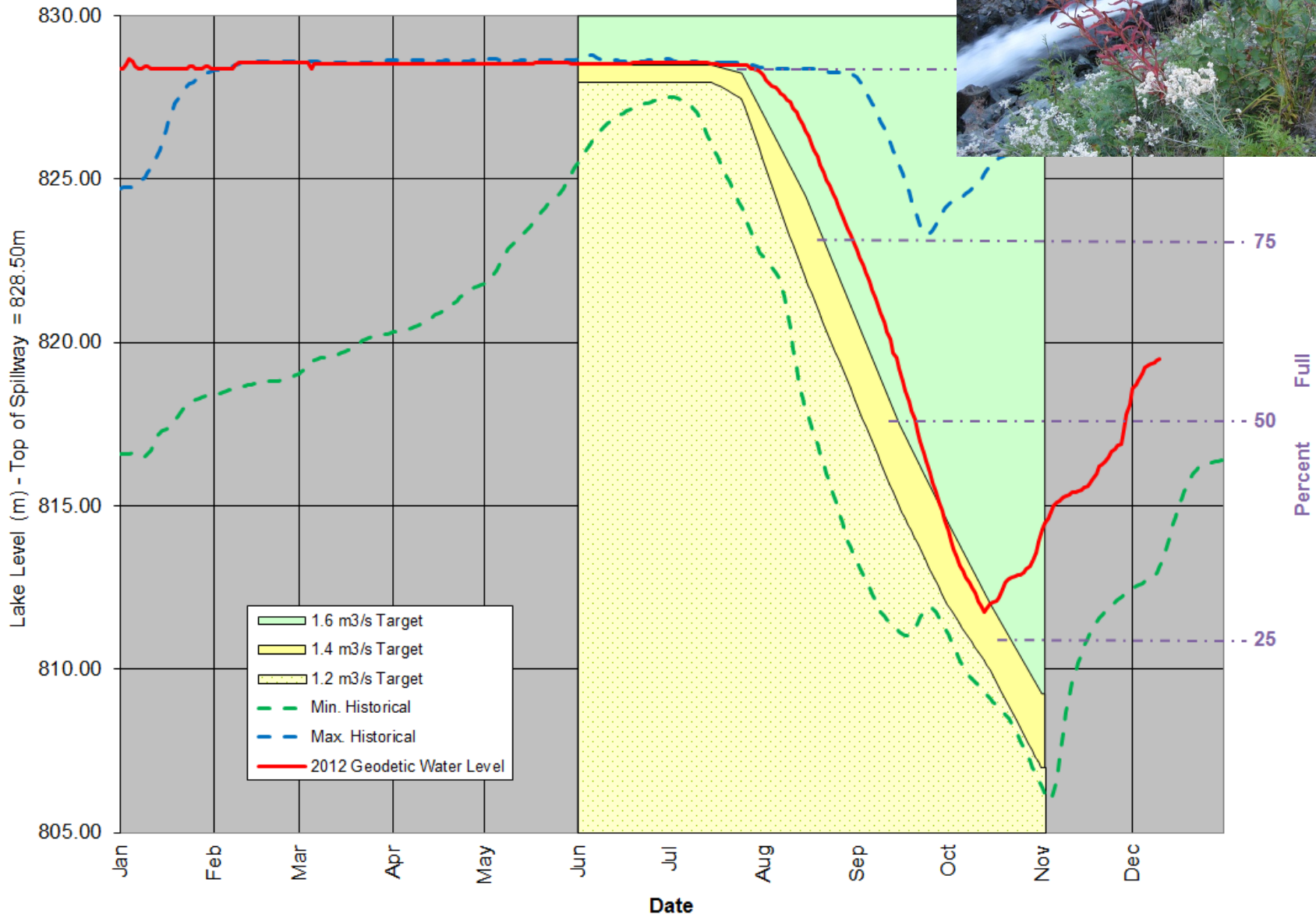
2012 Arrowsmith Dam Lake Levels - Provisional Operating Rule Curve
